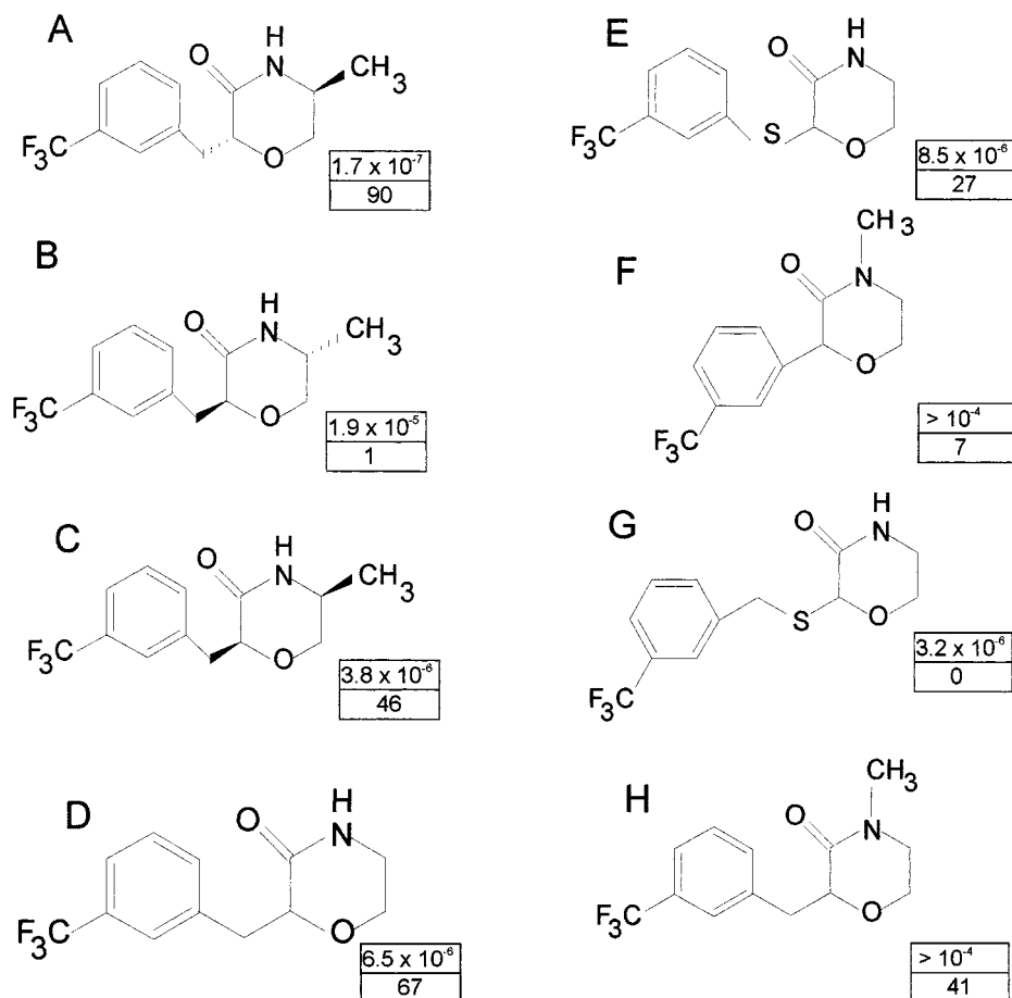
Figure 1. Structures of ketomorpholine derivatives, their I_{50} values (M) for inhibition of phytoene desaturase (top value) and averaged herbicidal activity at 1000 \text{ g ha}^{-1} (bottom value).
